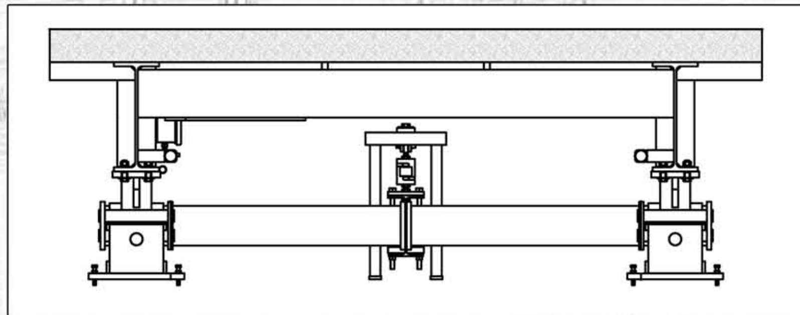
Electro-Mechanical Pit-Type - Concrete Deck
